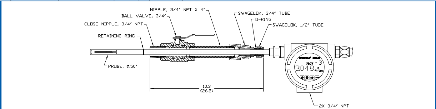
Figure 7: Crank Retractor - NPT 600 psig (41.4 barg); ANSI 150 & ANSI 300
