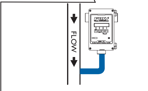
(F3) Flow Down - Meter Right
