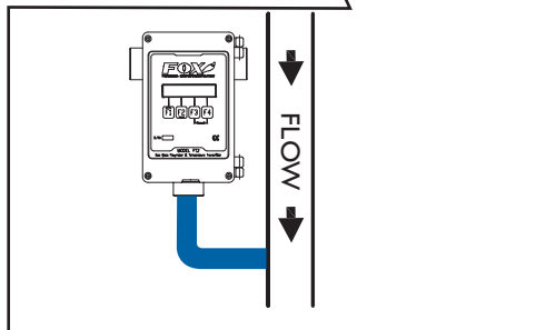
(F4) Flow Down - Meter Left
